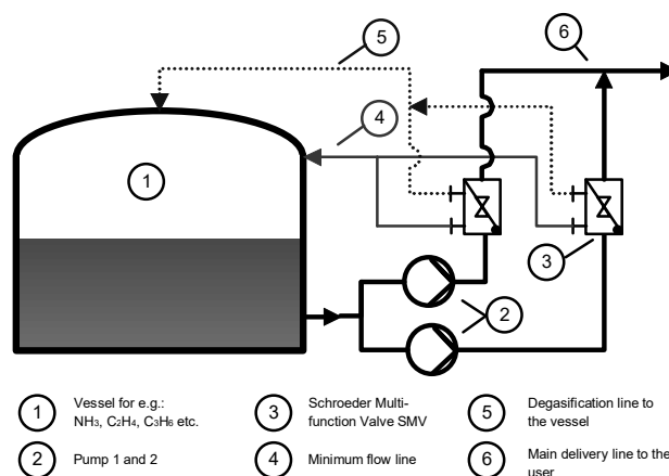
Figure 2 Delivery of easily boiling fluids
