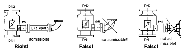
Figure 3 Mounting with straight pipe piece
