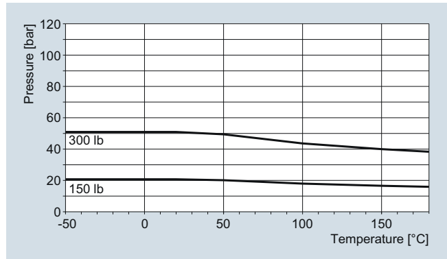
ASME-Flanges stainless steel AISI 326Ti/1.4571 to DN 100 (4")
